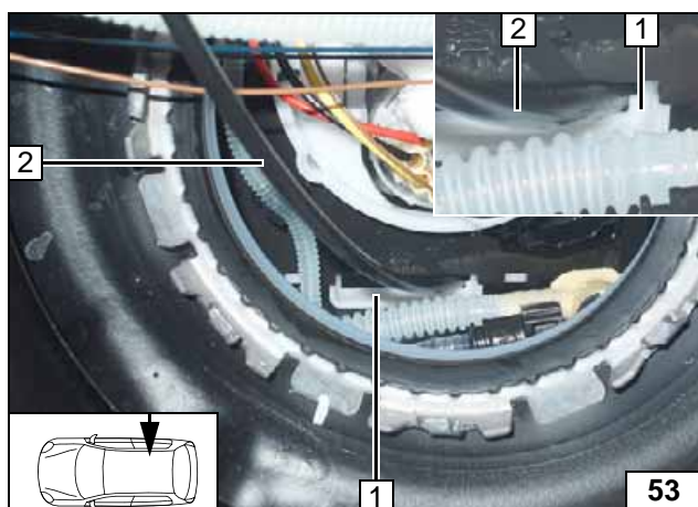
1 Plastic tab
