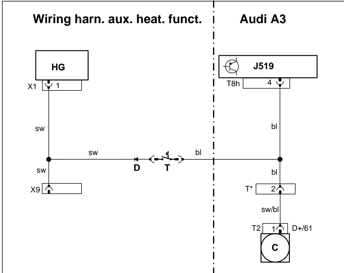
Wiring Diagram for Auxiliary Heating Function Audi A3
