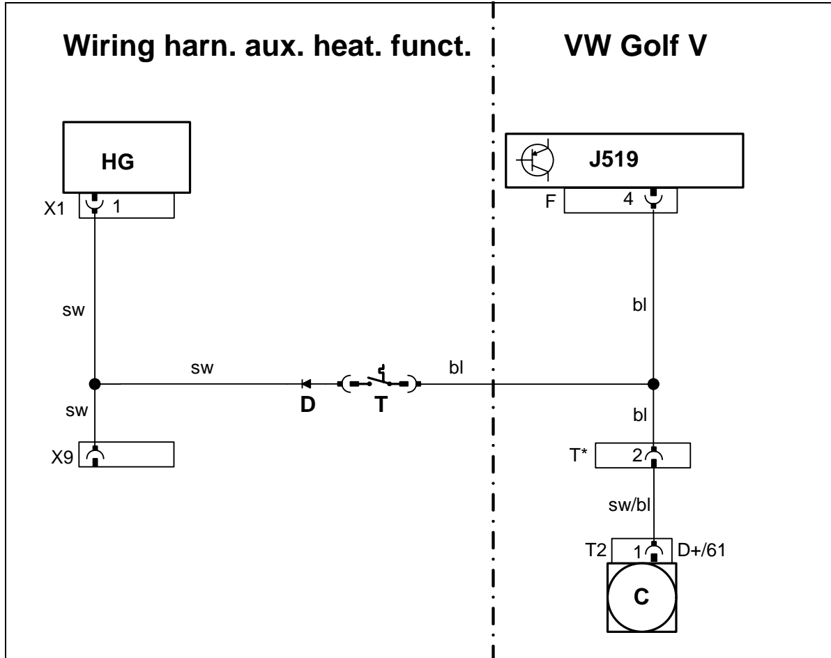
Wiring Diagram for Auxiliary Heating Function Golf V
