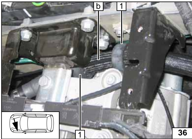
Position black (sw) rubber isolator 1 [2x]. Ensure sufficient distance to neighbouring components.
